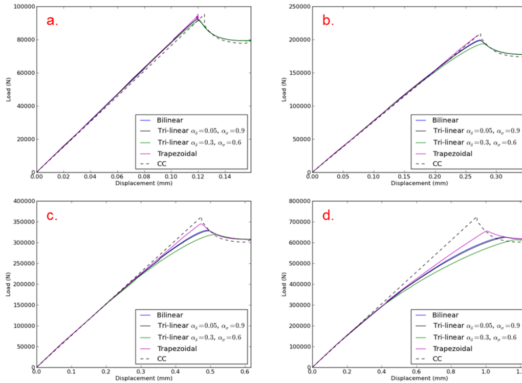
Figure 4. Comparison of load versus displacement curves between the coupled criterion (CC) and different cohesive zone models (CZM) with \sigma_C = 1 MPa and (a.) G_C = 1 \text{ J/m}^2 , (b.) G_C = 5 \text{ J/m}^2 , (c.) G_C = 15 \text{ J/m}^2 , (d.) G_C = 60 \text{ J/m}^2
